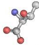
L-threonine (Thr, T)
